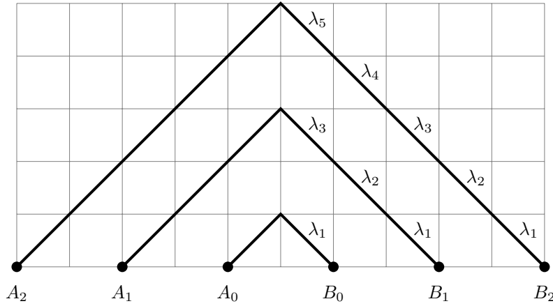
Figure 7.8: The unique nonintersecting (n + 1) -path in \text{NI}(A \rightarrow B^+) for the case n = 2 .
